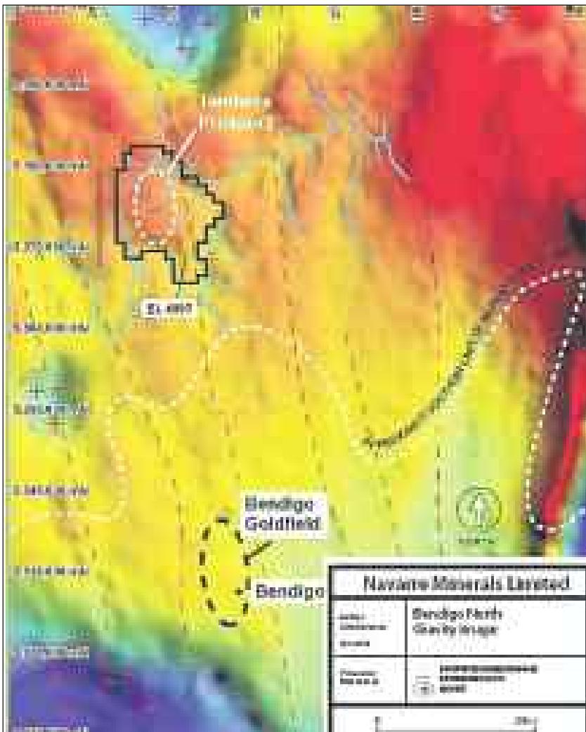
Tenement on an interpretation of the regional gravity image showing relationship of the Tandarra Prospect to the Bendigo Goldfield.
